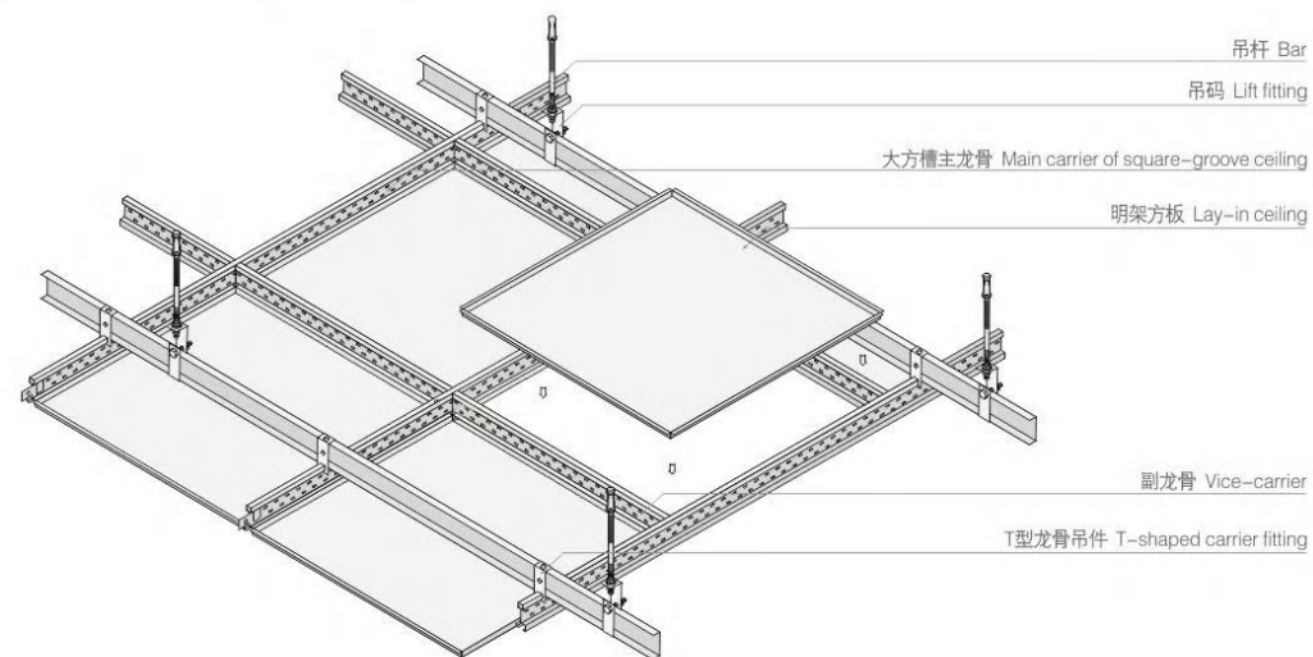
明架方板安装结构图 Structure Diagram of Lay-in Ceiling
