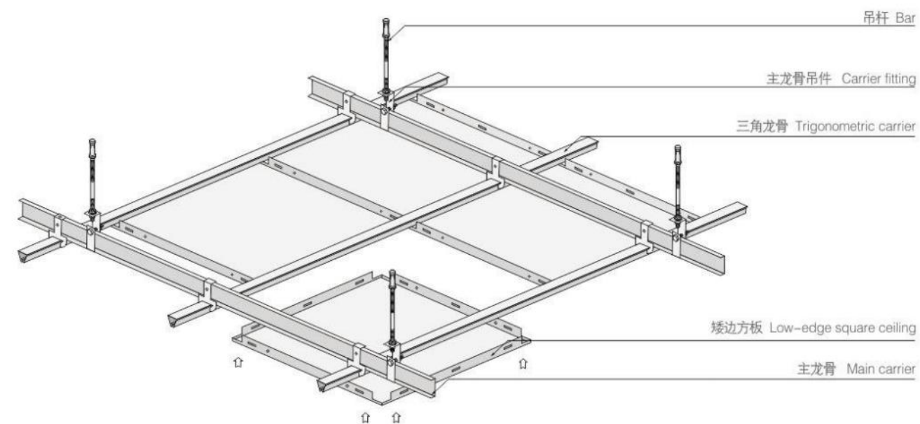
矮边暗架方板安装结构图 Structure Diagram of Low-edge Clip-in Ceiling
