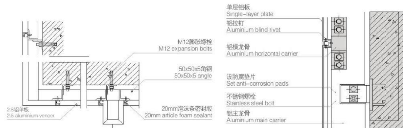
幕墙墙面转角大样图 General Graphic of Curtain Wall Corner
