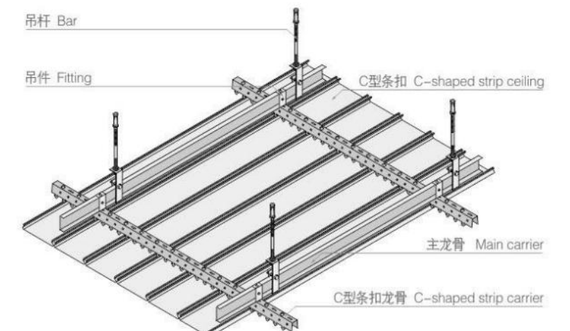
C型条扣龙骨拼装示意图 The Drawing of Installation of C-shaped Strip Carrier
