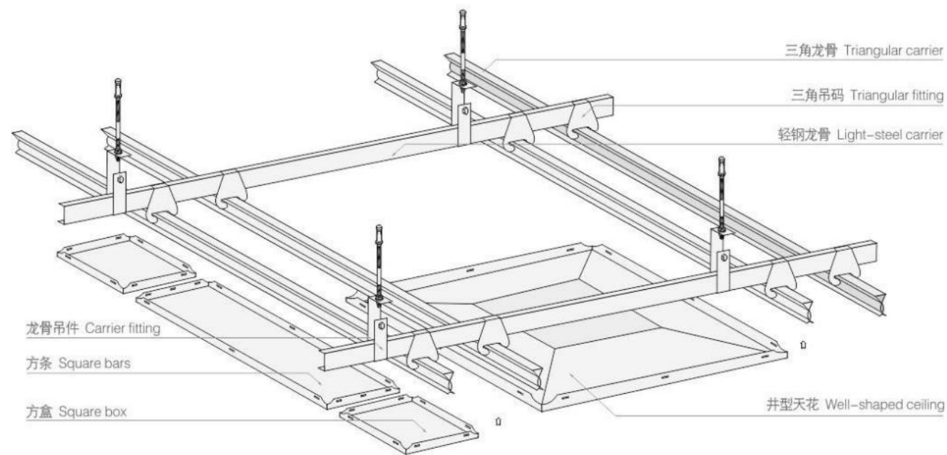
井型天花结构图 Structure Diagram of Well-shaped Ceiling
