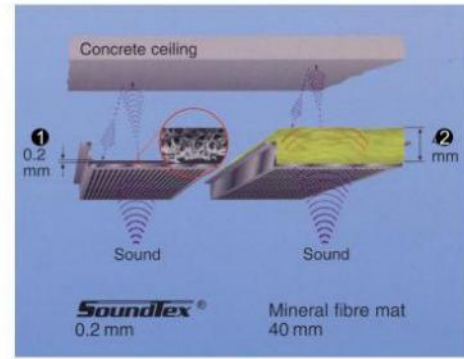
声音在吸音材料上的能量转换过程 The transformation process of sound, which is on sound-absorbing materials.
