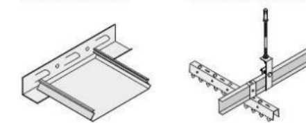
修边角拼装示意图 The Drawing of Installation of Wall Edge Corner
