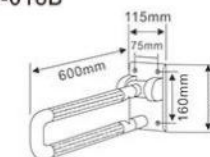
HS-018B
