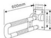
HS-018C
