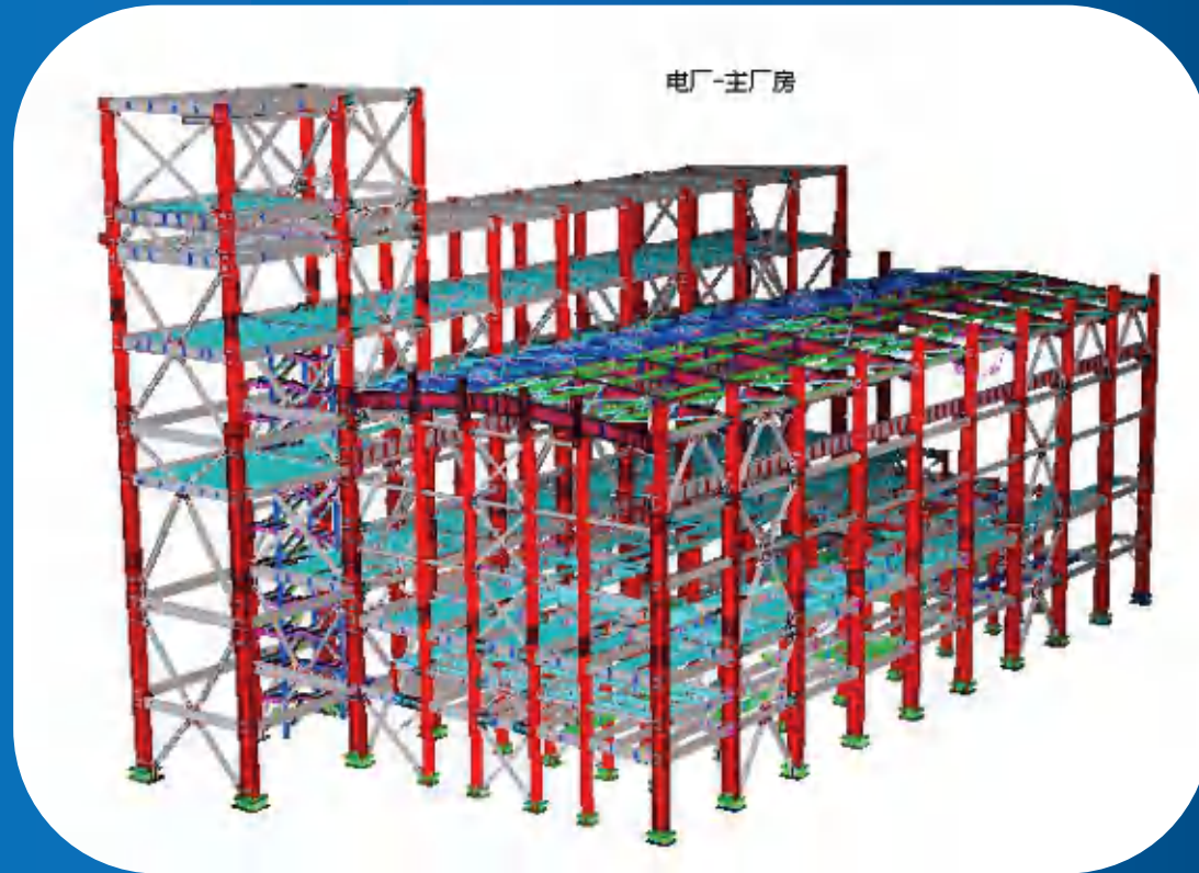
Power plant model
