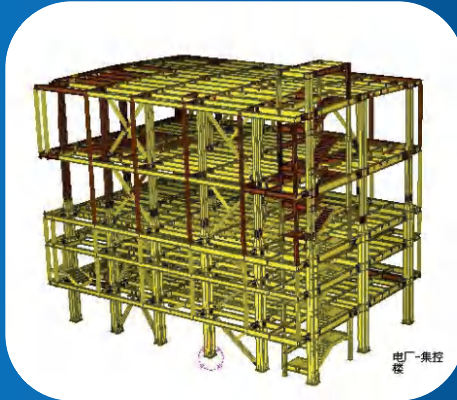
Integrated control building model
