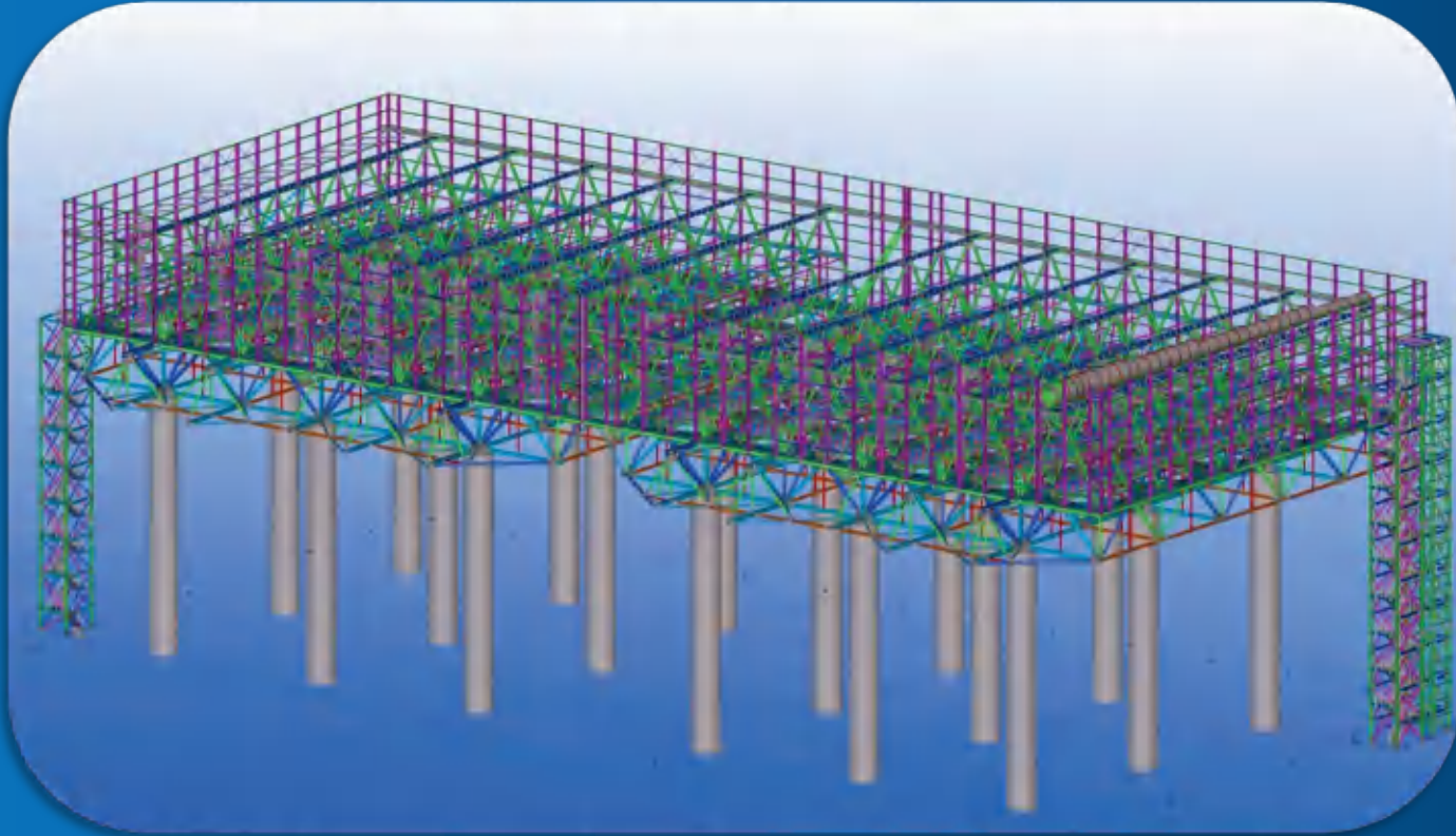
Air-cooled island model picture
