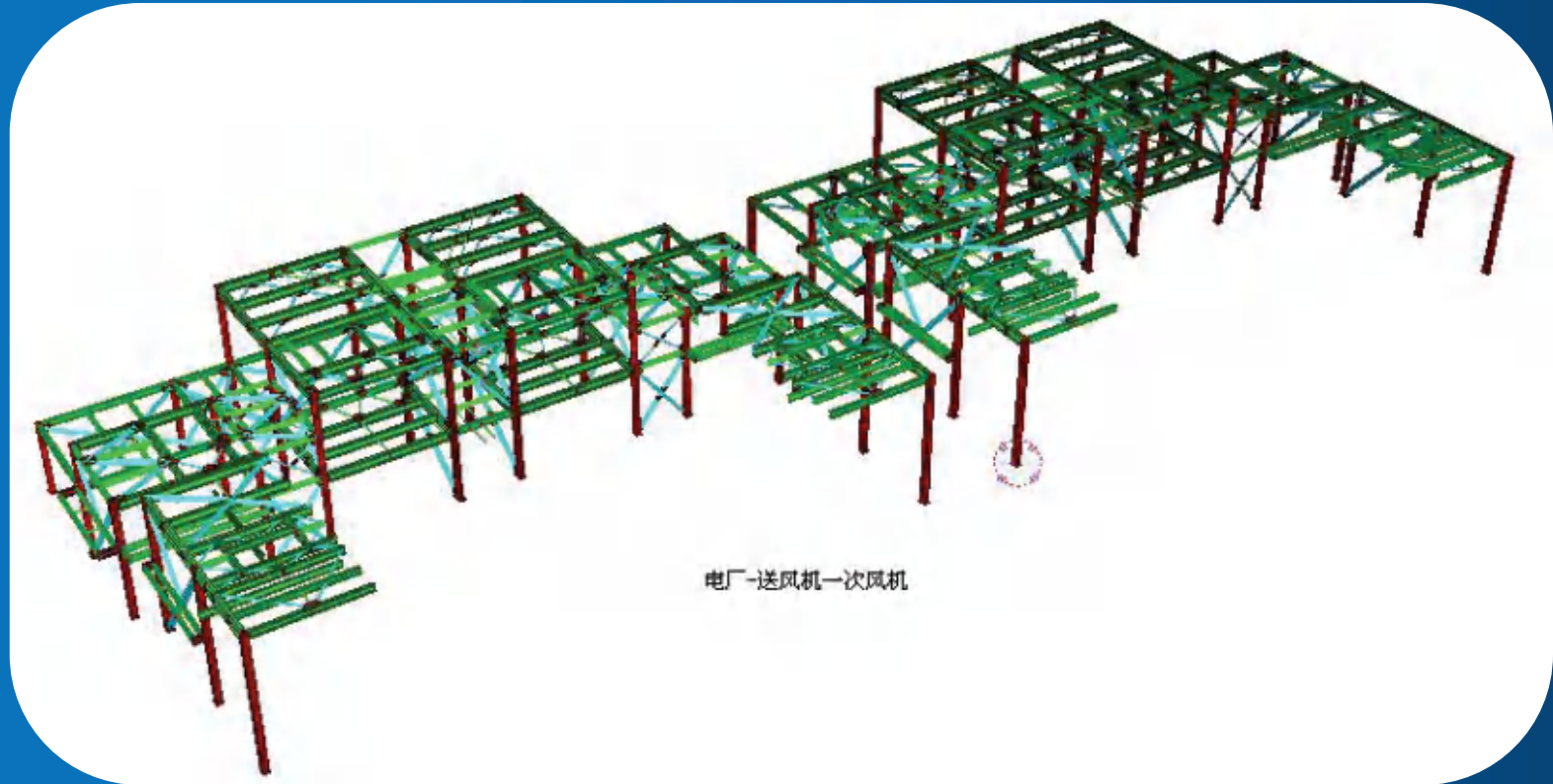
Blower model
