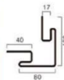
外角 Outside Corner Post(Ha 4) Length: 2.95m Pieces per carton: 6 Coverage per carton: 17.70m
