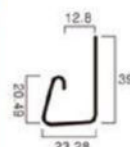
J条 J-channel(Ha 2) Length: 2.95m Pieces per carton: 32 Coverage per carton: 94.40m
