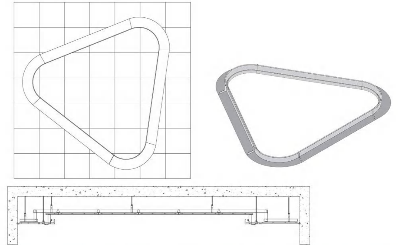
* YCDB-011 Bilaminar triangle model
