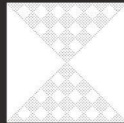
Description: \varnothing 3 diagonal match punching aluminum square plate Code:YC6008
