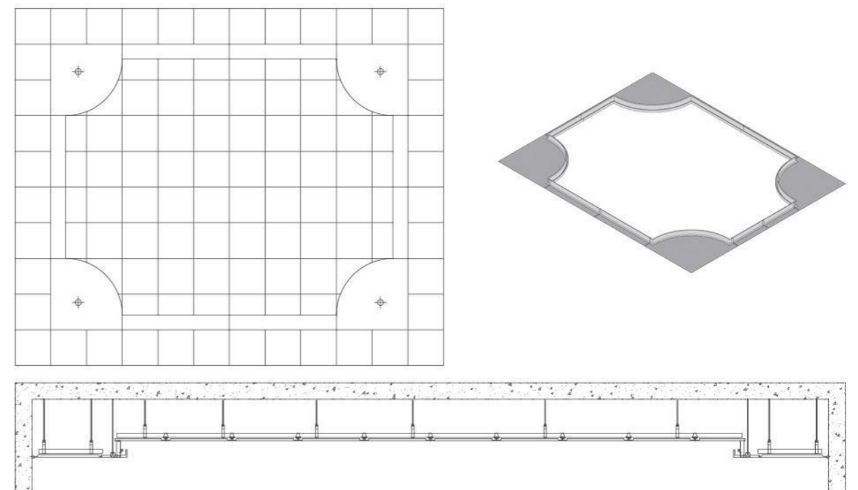
* YCDB-015 Arc corner panel
