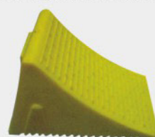
Model 型号:LZL-DWQ-08 Sizen 尺寸:190x105x125mm Material:plastic 材质:塑料
