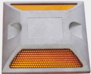
型号(model):LZL-DD-03 材料(material):塑料(plastic); PC反光片(PCreflective sheeting) 规格(specification):单面或双面反光 (single or double-side) 尺寸(size):100 × 100 × 20mm
