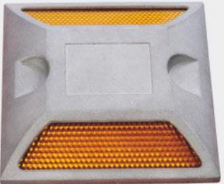
型号(model):LZL-DD-04 材料(material): 全铝(complete aluminium); PC反光片(PCreflective sheeting) 规格(specification):单面或双面反光 (single or double-side) 尺寸(size):100 × 100 × 20mm
