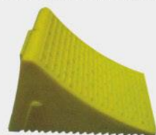
Model 型号:LZL-DWQ-08 Sizen 尺寸:190x105x125mm Material:plastic 材质:塑料
