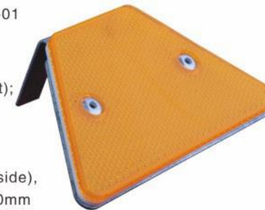
材料(material): 钢支架或者塑料支架 (Steel or plastic bracket); PC反光片(PC reflector) 规格(specification): 双支单面(double bracket single-side) 尺寸(size): 120 × 70 × 50mm
