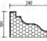
EPS-40 规格: 240 X 160
