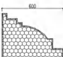
EPS-42 规格: 600 X 450
